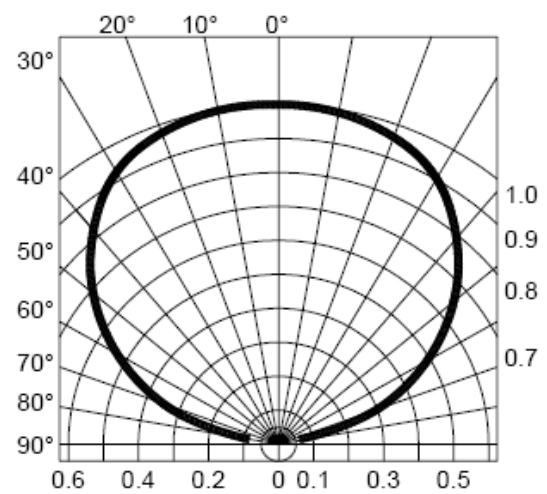
Radiation Diagram
