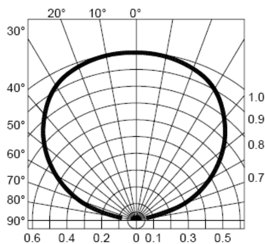
Radiation Diagram
