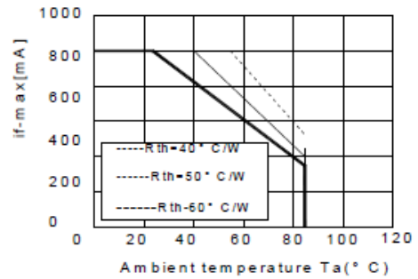
Fig.6 Maximum Driving Forward DC Current vs. Ambient Temperature (Derating based on T_J max. = 115^\circ\text{C} )
