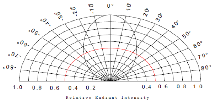
Fig.7 Radiation diagram
