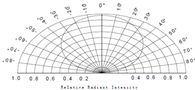
Fig.7 Radiation diagram
